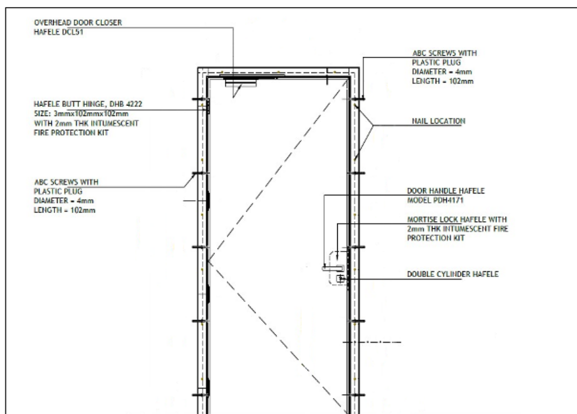
Figure 1. Specimen Layout
