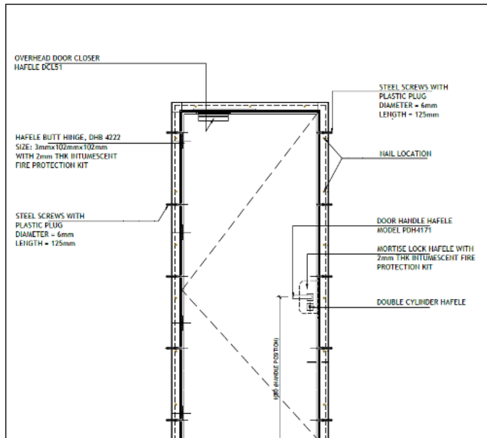
Figure 1. Specimen layout
