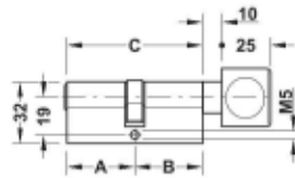
Thumbturn cylinder
